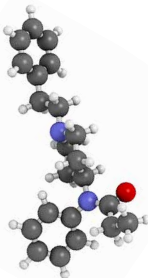
▲ Fentanylmolekyl
